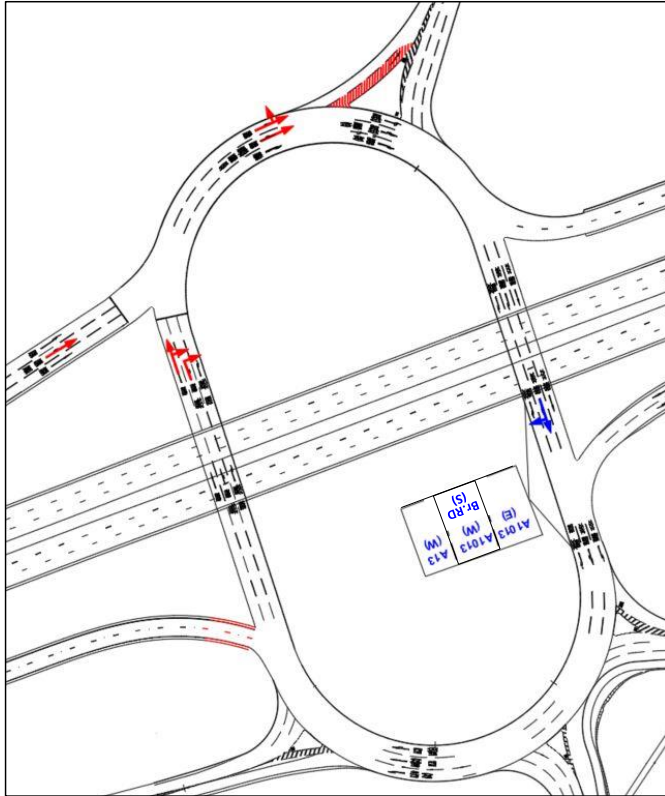
Plate 3.6 Modified Lane Markings at Roundabout
