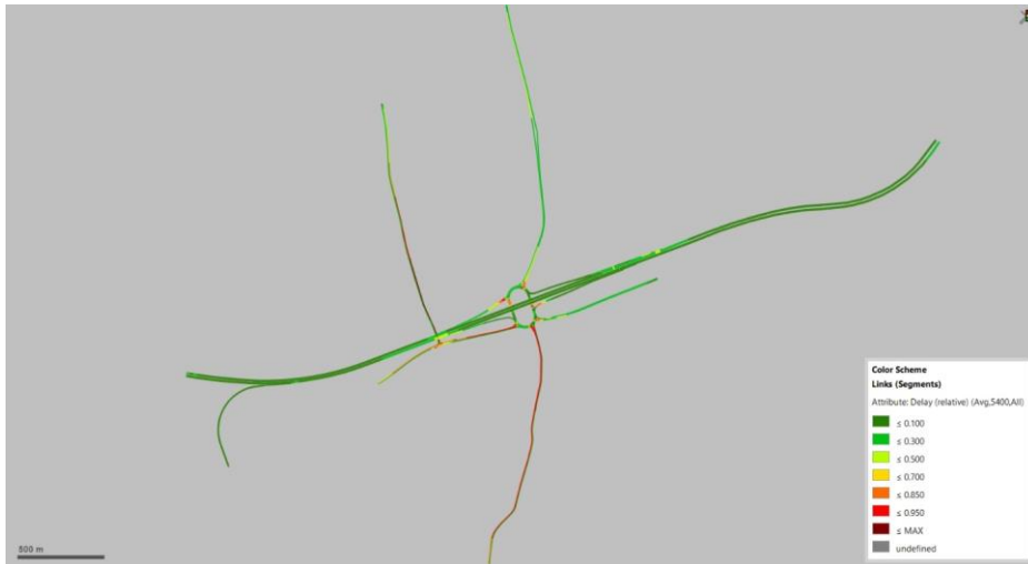
Plate 4.6 Relative Delay Plot (2030 DS 08:00 – 09:00)
