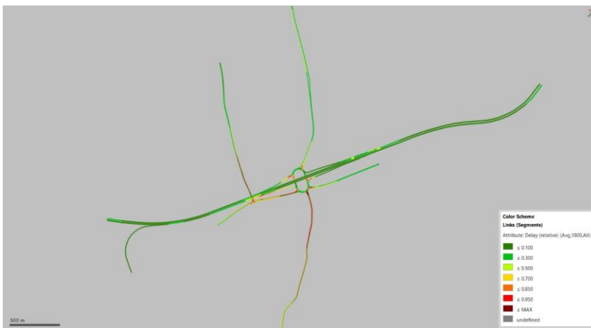
Plate 4.10 Relative Delay Plot (2045 DS 07:00 – 08:00)
